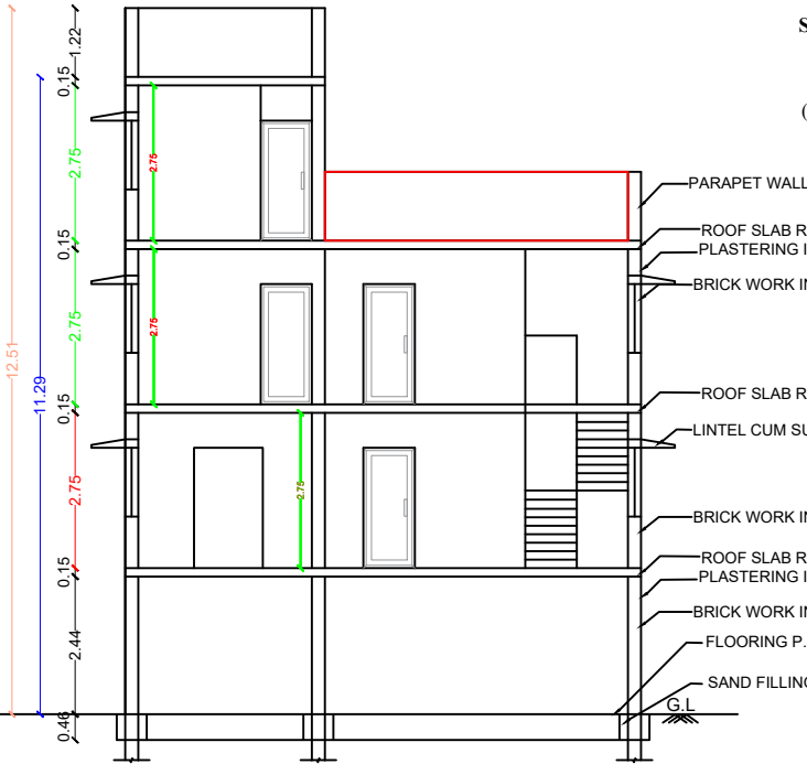
SECTION "A-B"
