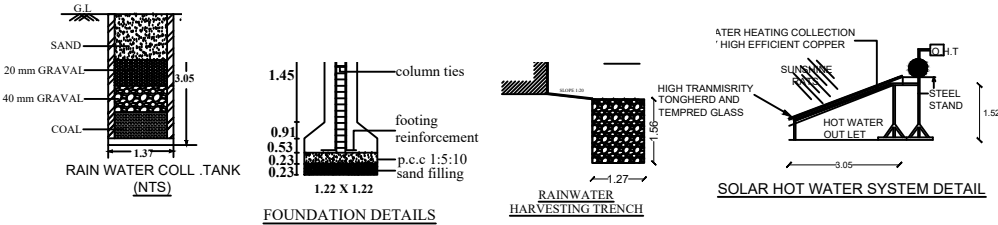
FOUNDATION DETAILS
