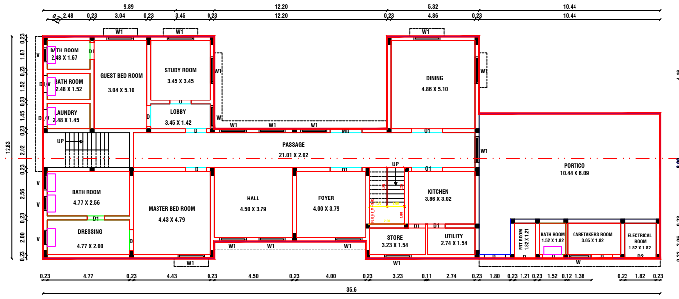
PROPOSED GROUND FLOOR
