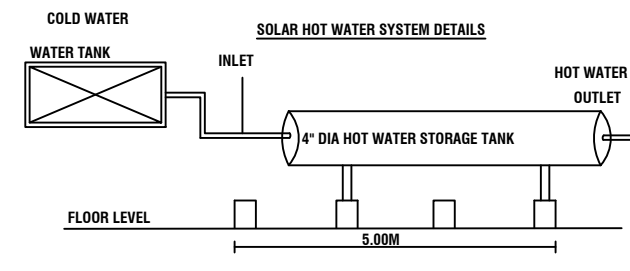
SOLAR HOT WATER SYSTEM DETAILS
