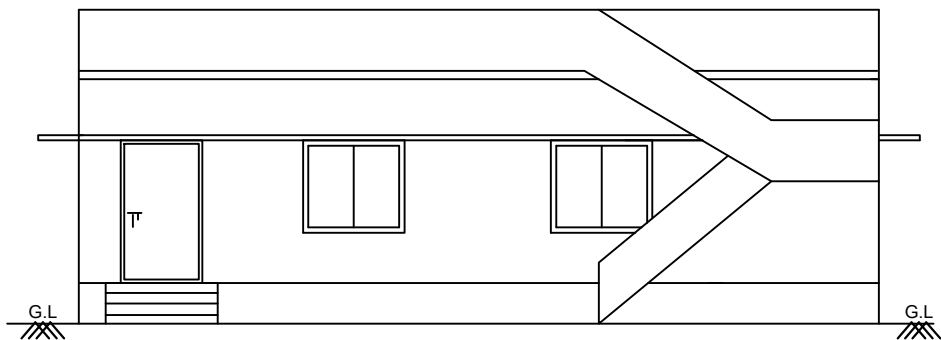
FRONT ELEVATION
