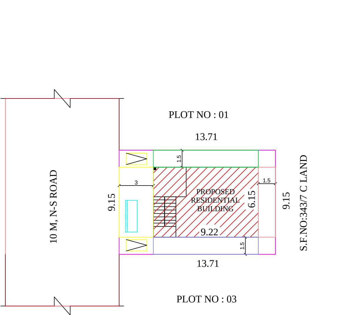
SITE PLAN
