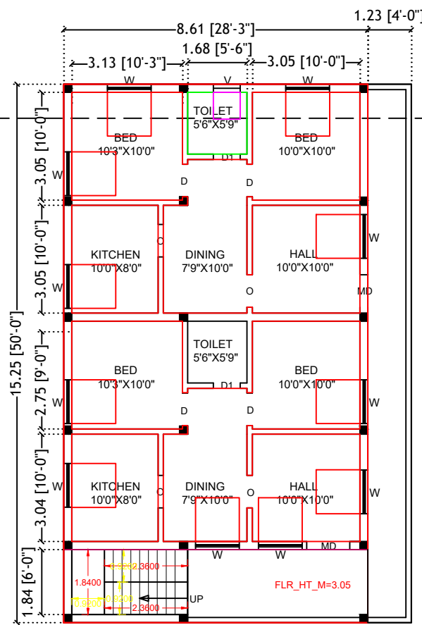
FIRST FLOOR PLAN (EXISTING BUILDING)
