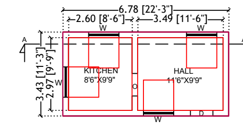
GROUND FLOOR PLAN (PROPOSED BUILDING)
