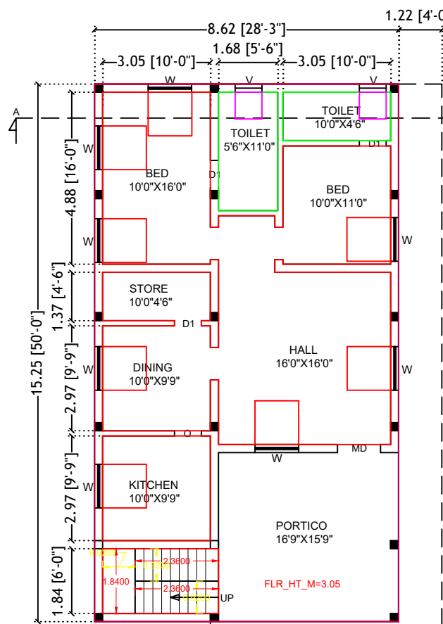
GROUND FLOOR PLAN (EXISTING BUILDING)
