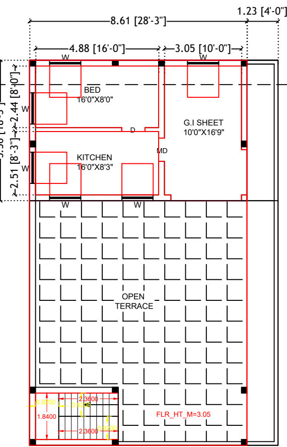
SECOND FLOOR PLAN (PROPOSED BUILDING)
