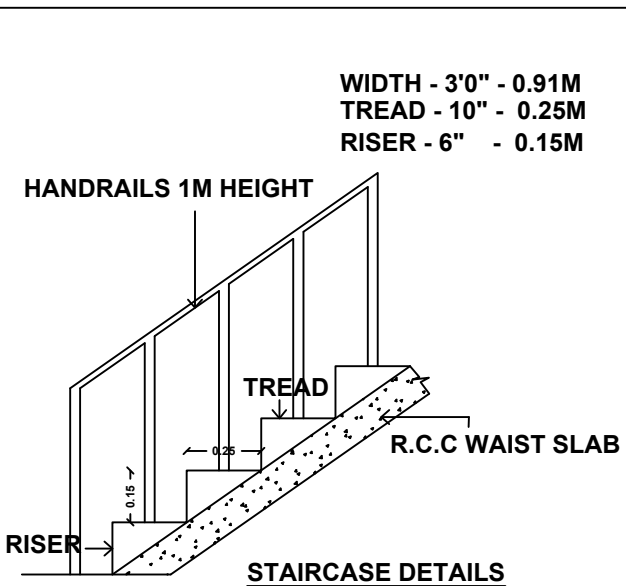
STAIRCASE DETAILS
