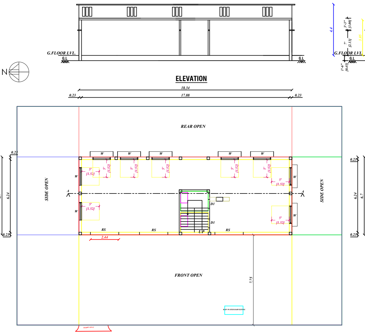
15 m WIDE KARUR - DINDIGUL MAIN ROAD GROUND FLOOR PLAN
