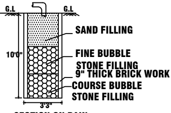
SECTION ON RAIN WATER COLLECTION TANK
