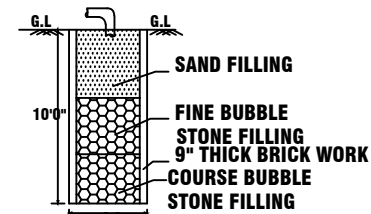
RAIN WATER COLLECTION TANK COLLECTION OF RAIN WATER FROM BUILDING
