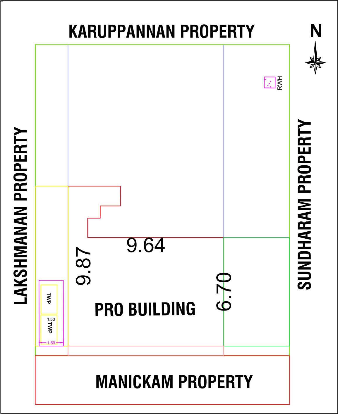
SITE PLAN
