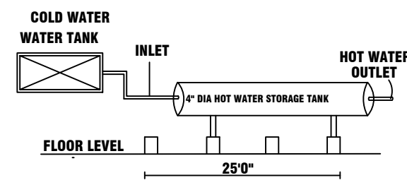
SOLAR HOT WATER SYSTEM DETAILS
