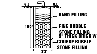
SECTION ON RAIN WATER COLLECTION TANK
