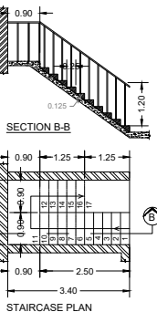
STAIRCASE PLAN
