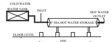
SOLAR HOT WATER SYSTEM DETAILS
