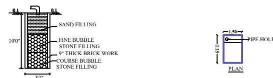
SECTION ON RAIN WATER COLLECTION TANK
