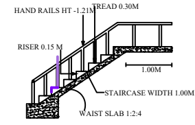
STAIRCASE DETAILS
