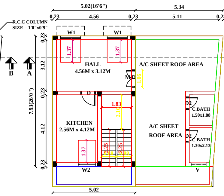
FLOOR-02 PRO.SECOND FLOOR PLAN
