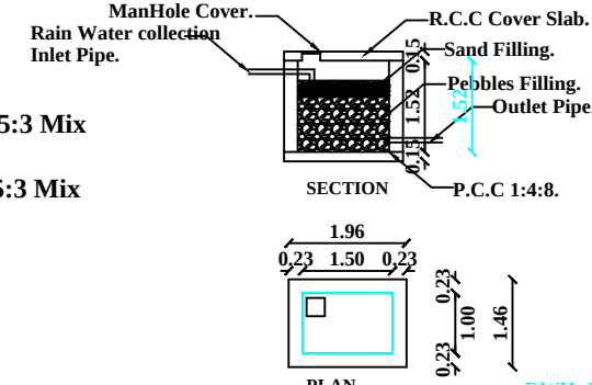
DETAILS OF COLLECTION SUMP FOR WATER HARVESTING FOR ROOF TOP RAIN WATER.
