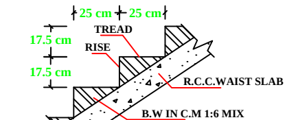
SECTION OF STAIRCASE
