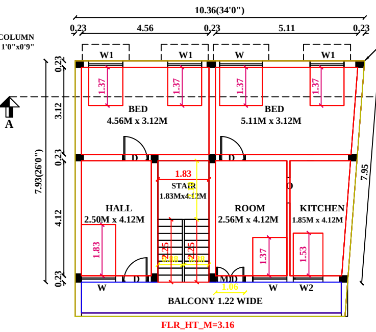
FLOOR-01 PRO.FIRST FLOOR PLAN
