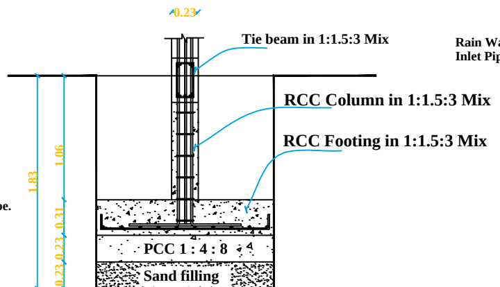
CROSS SECTION ON 'C - C'
