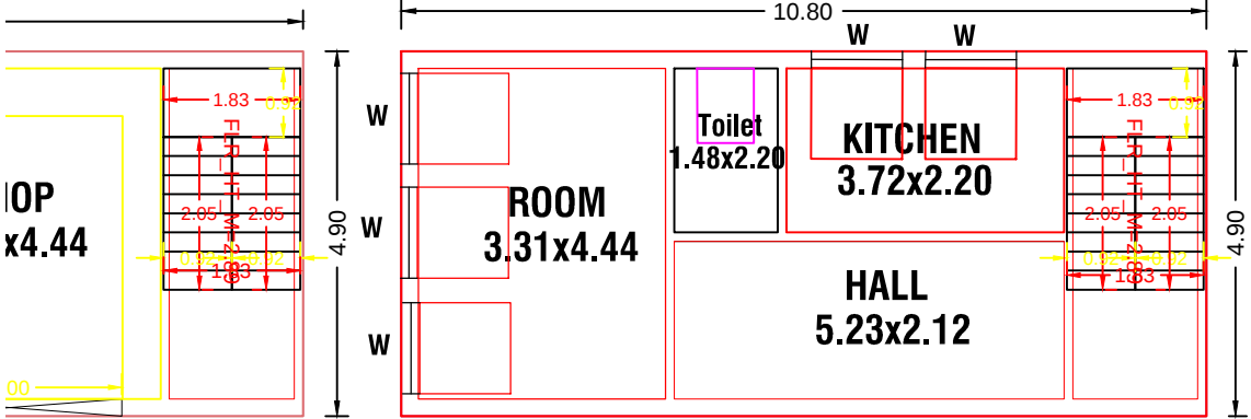
PRO., FIRST FLOOR PLAN
