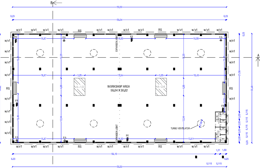
BLOCK -1 AND 2 PRO.GROUND FLOOR PLAN (TYPICAL FLOOR)
