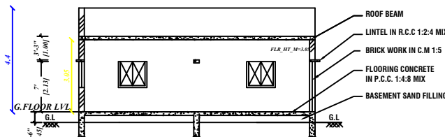
SECTION ON-AA
