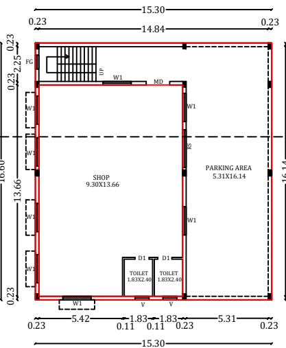
FLOOR-GROUND PRO.GROUND FLOOR PLAN
