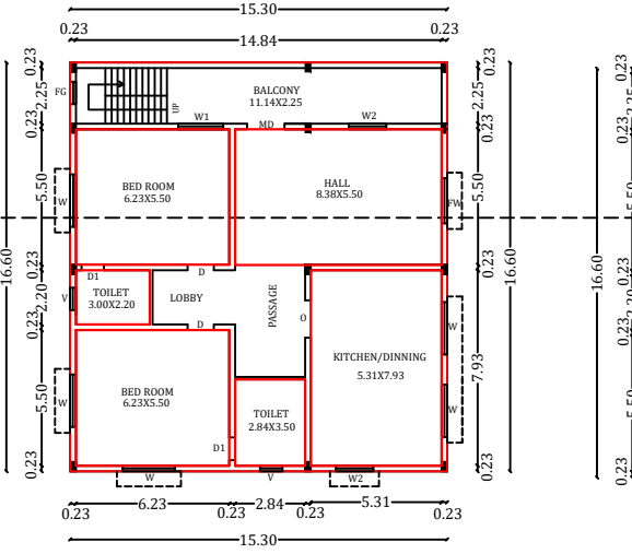
FLOOR-FIRST PRO.FIRST FLOOR PLAN
