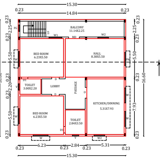
FLOOR-SECOND PRO.SECOND FLOOR PLAN
