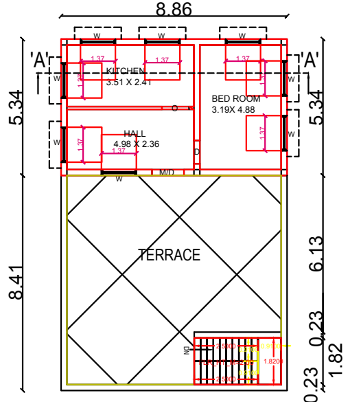
FLOOR-FIRST PRO. FIRST FLOOR PLAN
