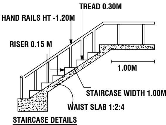
STAIRCASE DETAILS
