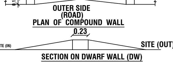
SECTION ON DWARF WALL (DW)
