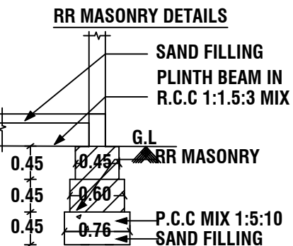
RR MASONRY DETAILS
