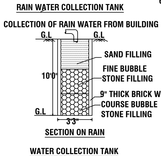
SECTION ON RAIN WATER COLLECTION TANK
