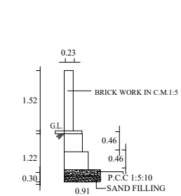
CROSS SEC. OF COMPOUND WALL
