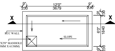
DRINKING WATER SUMP - PLAN
