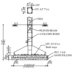
TYPICAL SECTION OF FOOTING
