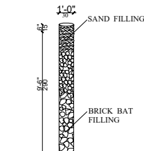
PERCOLATION PIT FOR RAIN WATER HARVESTING
