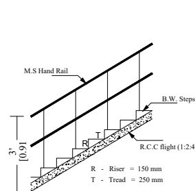
STAIRCASE DETAIL SCALE 1:50
