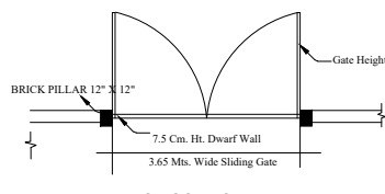
PLAN OF COMPOUND WALL
