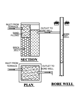
RAIN WATER HARVESTING DETAIL
