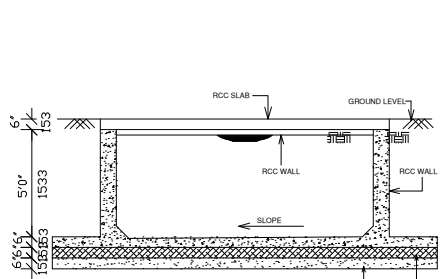
SECTION AT 'XX'
