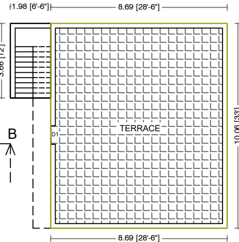
TERRACE PLAN
