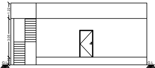
FRONT ELEVATION
