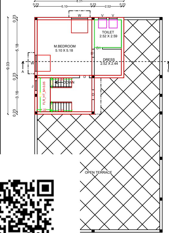
SECOND FLOOR
