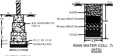
FOOTING DETAIL
