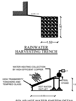
SOLAR HOT WATER SYSTEM DETAIL
