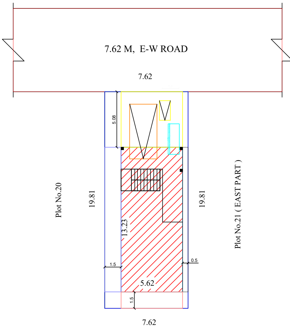
GARDEN CITY -I ,LAYOUT
