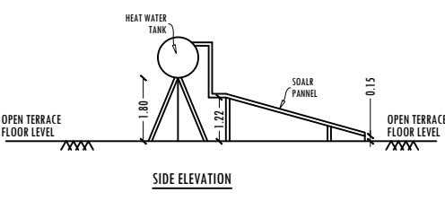
SIDE ELEVATION
