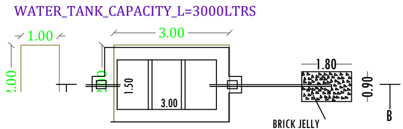
TANK & DISPERSION TRENCH DETAILS
