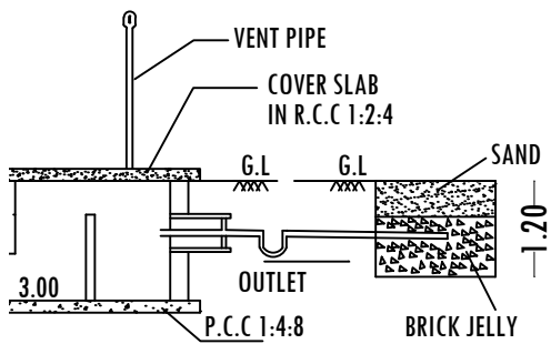
SECTION-AB
