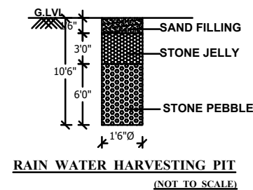
RAIN WATER HARVESTING PIT (NOT TO SCALE)
