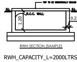
RWHT_CAPACITY_L=2000LTRS
