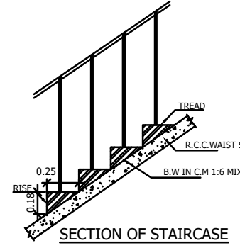
SECTION OF STAIRCASE (NOT TO SCALE)
