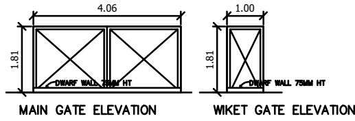
MAIN GATE ELEVATION WCKET GATE ELEVATION
