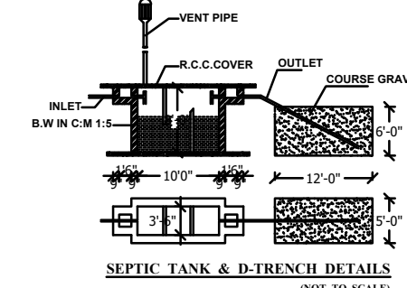
SEPTIC TANK & D-TRENCH DETAILS (NOT TO SCALE)
