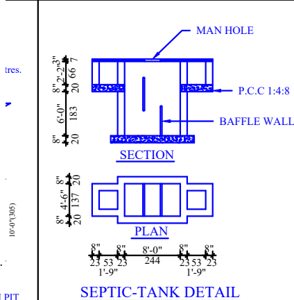
SEPTIC-TANK DETAIL
