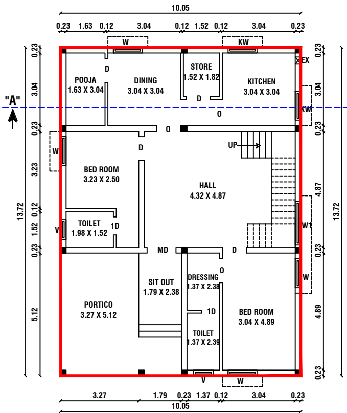
FLOOR - GROUND PRO. GROUND FLOOR PLAN
