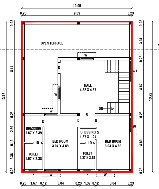
FLOOR - FIRST & TERRACE PRO. FIRST & TERRACE FLOOR PLAN
