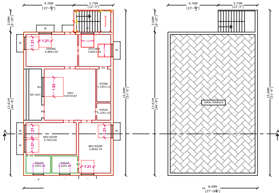
DR - TERRACE RACE FLOOR PLAN
