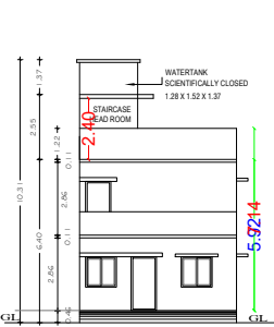
FRONT ELEVATION.
