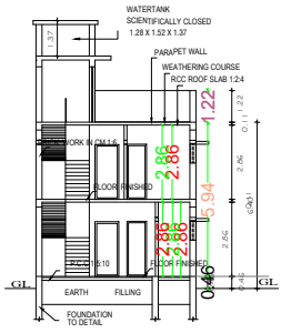
SECTION "AB"
