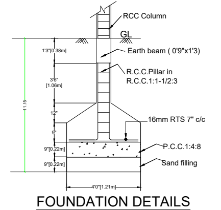
FOUNDATION DETAILS
