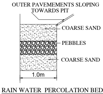
RAIN WATER PERCOLATION BED
