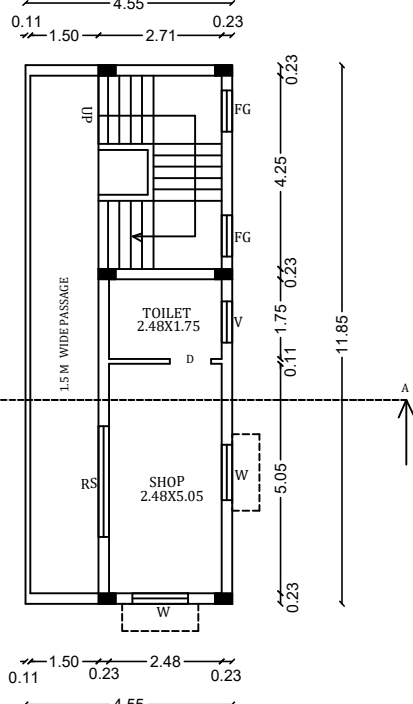
FLOOR-FIRST PRO.FIRST FLOOR PLAN
