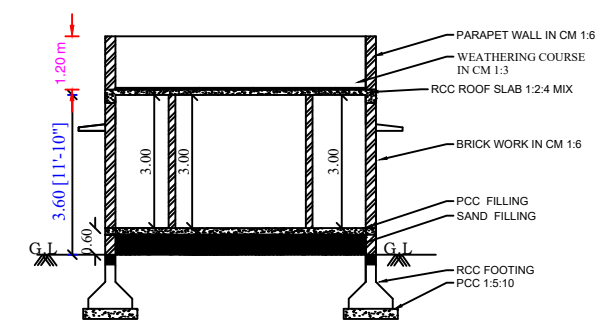
SECTION - "SR"
