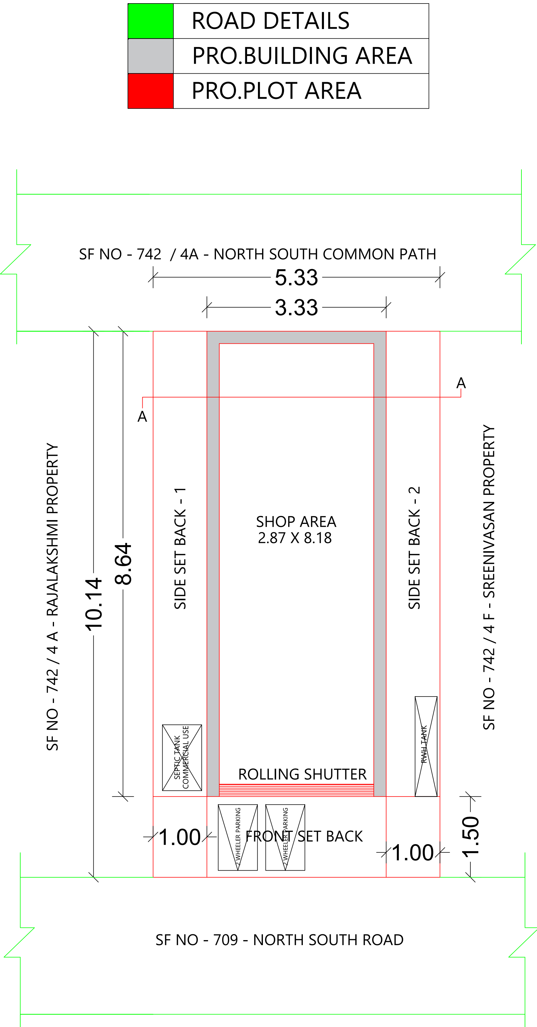
PROPOSED COMMERCIAL BUILDING - 1.NOS PLAN CUM SITE PLAN SCALE - 1:100
