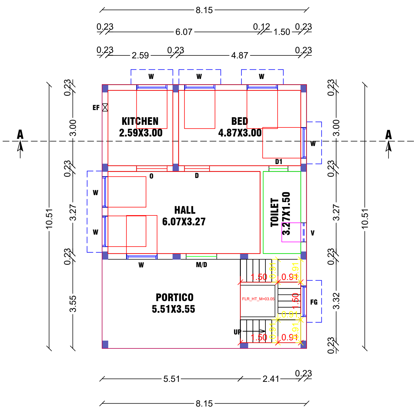
FLOOR-GROUND PRO.GROUND FLOOR PLAN
