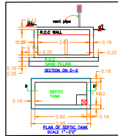
PLAN OF SEPTIC TANK SCALE 1"=2'0"
