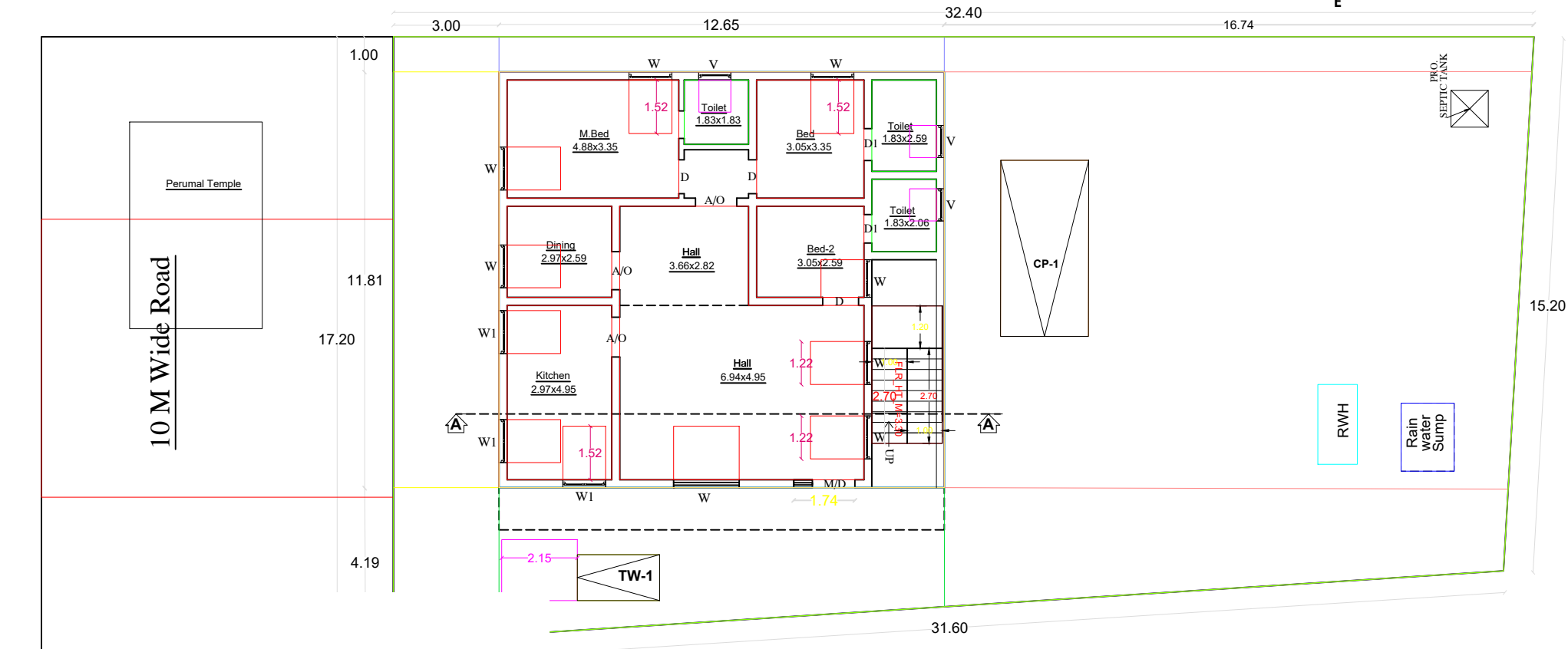
PLAN CUM GROUND FLOOR PLAN
