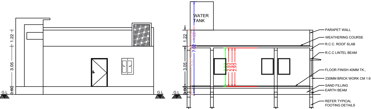
FRONT ELEVATION
