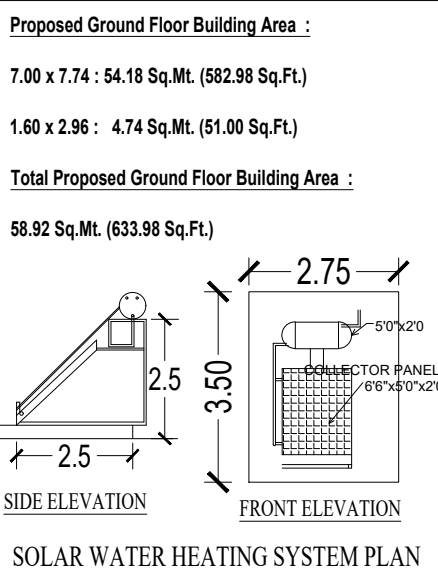
SOLAR WATER HEATING SYSTEM PLAN
