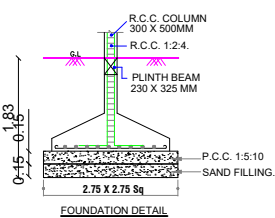
FOUNDATION DETAIL
