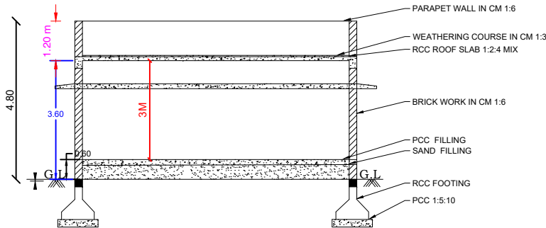
SECTION ON - "SR"
