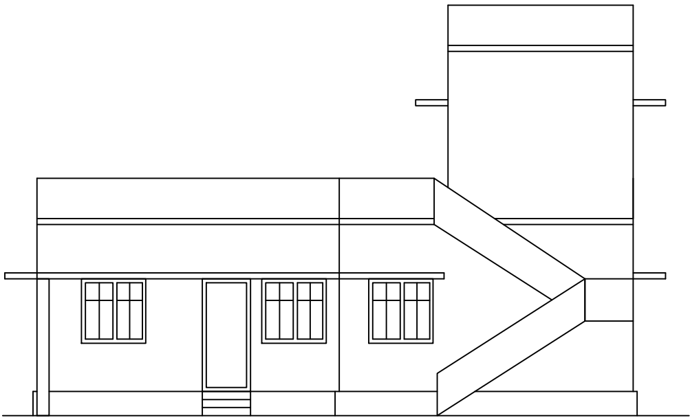
FRONT ELEVATION
