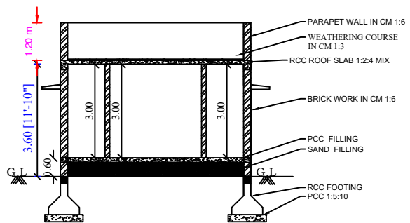
SECTION - "SR"
