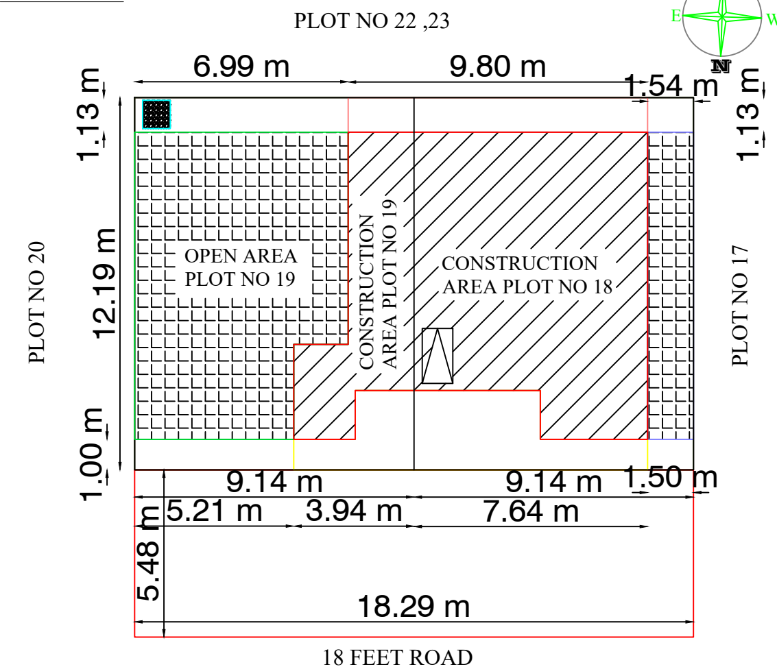
SITE PLAN
