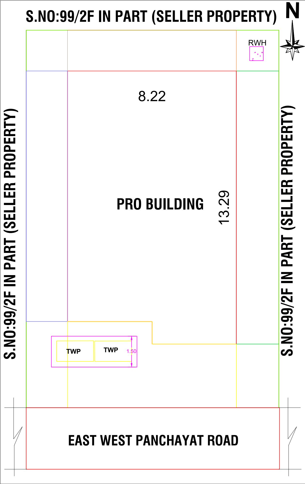
SITE PLAN
