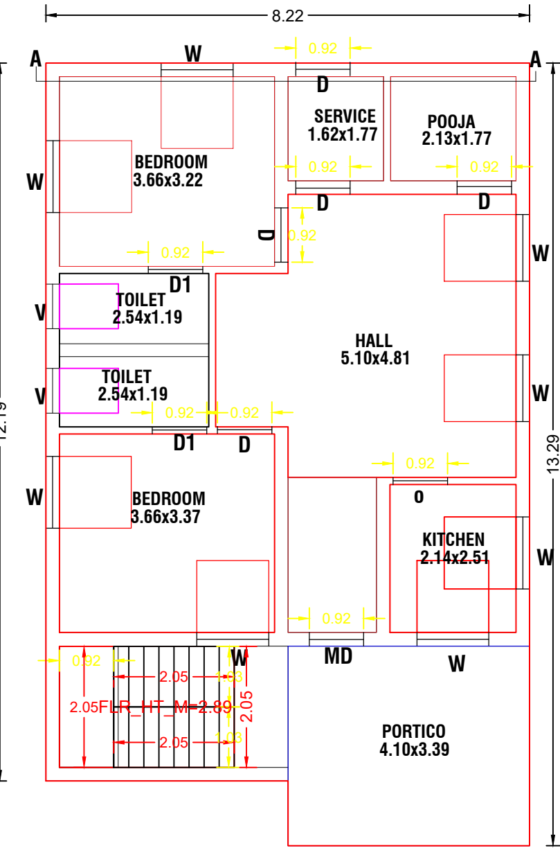
FLOOR PLAN
