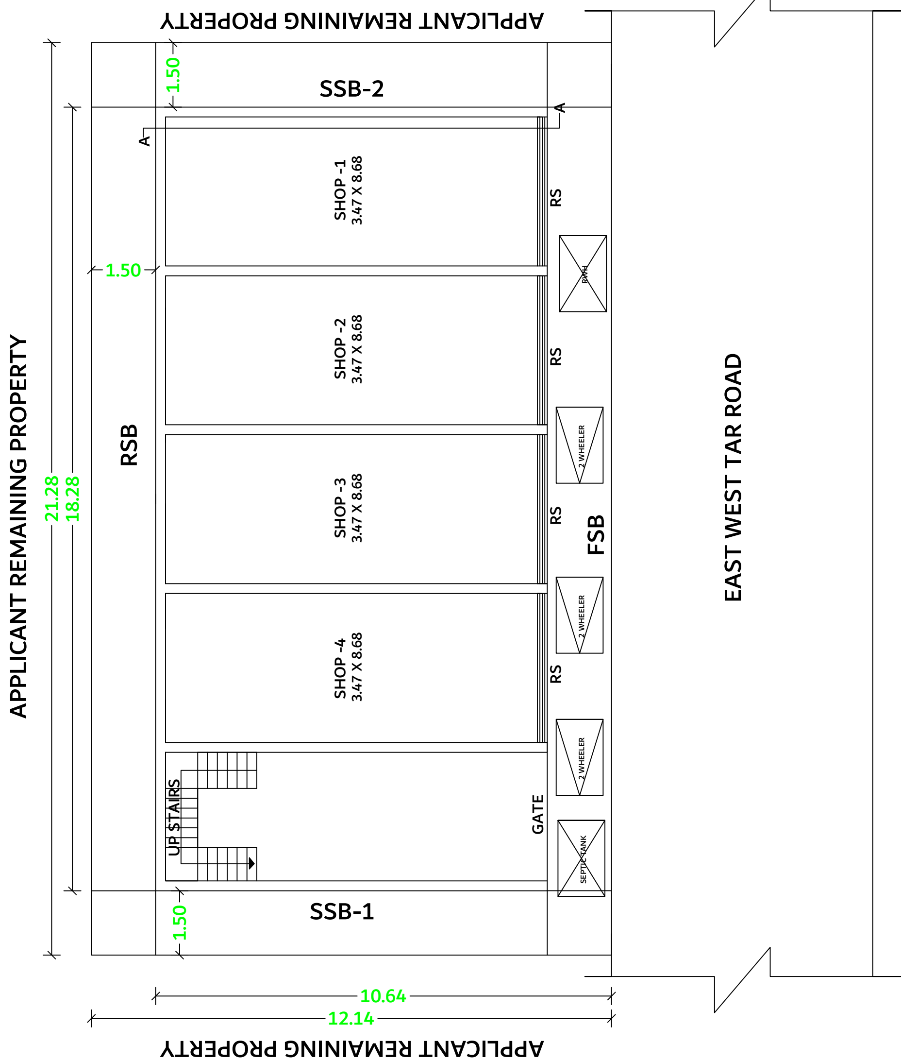
PROPOSED COMMERCIAL BUILDINGS - 4 NOS CUM SITE PLAN - SCALE - 1 : 100
