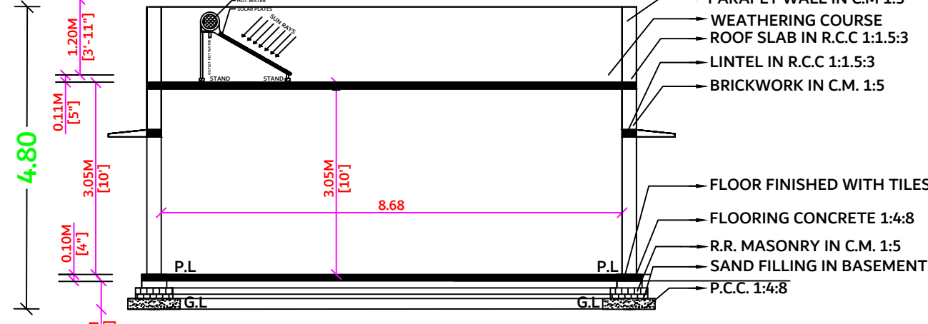
SECTION PLAN ON AA
