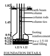
FOUNDATION DETAILS
