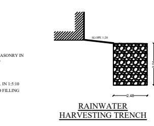
RAINWATER HARVESTING TRENCH
