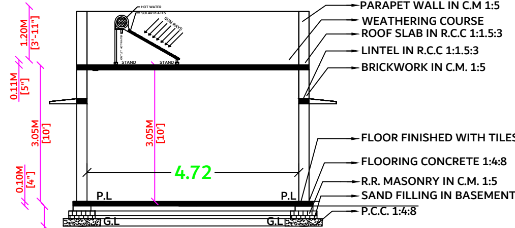
SECTION PLAN ON AA
