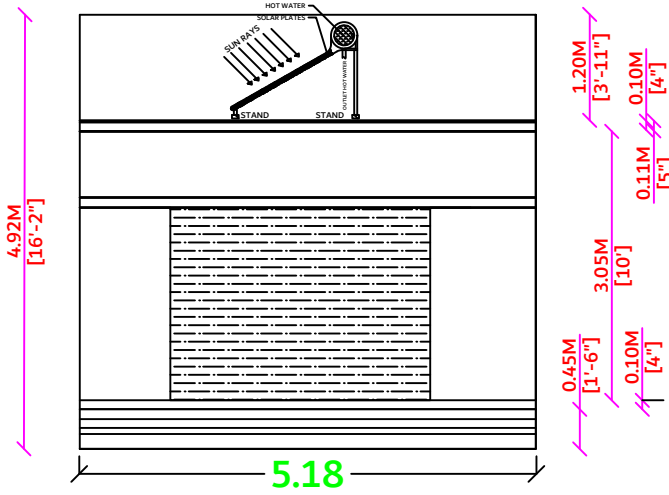
ELAVATION - SOUTH FACING
