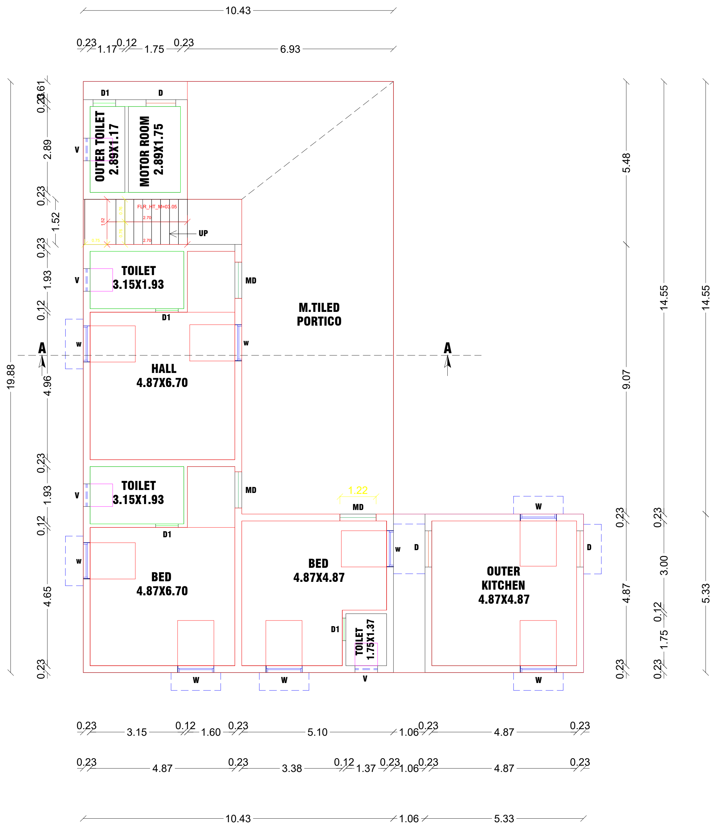
FLOOR-GROUND
