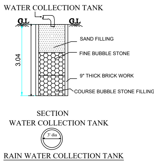
RAIN WATER COLLECTION TANK
