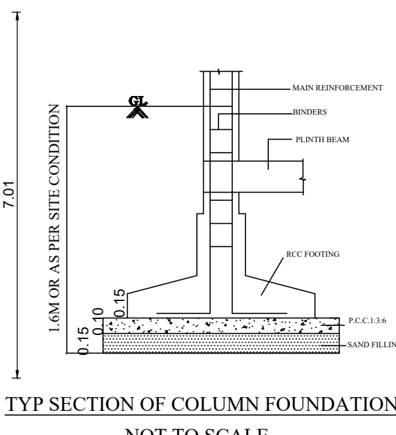
TYP SECTION OF COLUMN FOUNDATION
