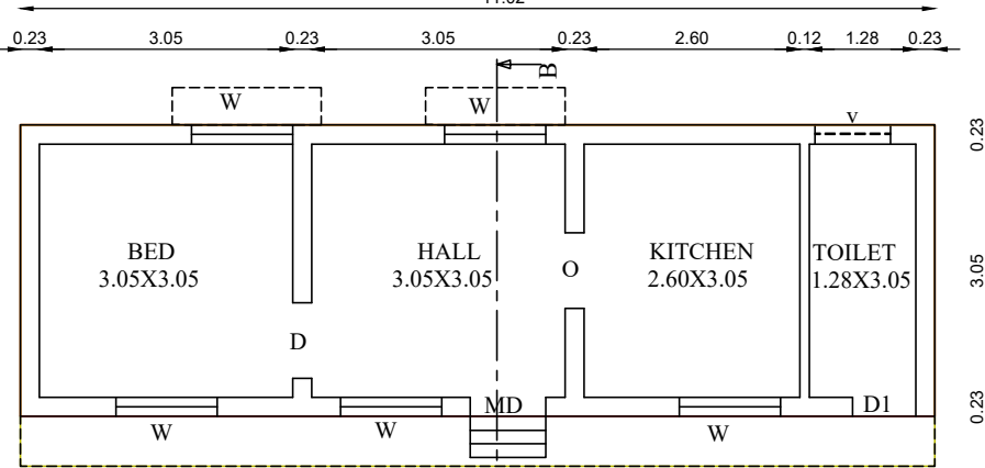
PRO.GROUND FLOOR PLAN BLOCK-2
