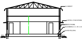
SECTION"A-B"
